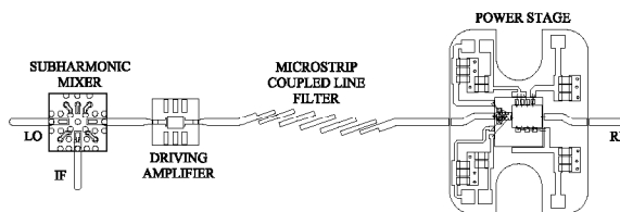
Figure 1: Designed modules configuration.
