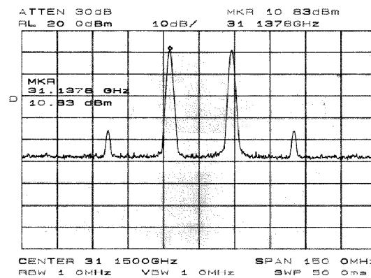
Figure 10: Two tone measurement example for the whole 31.15 GHz transmitter module. Single tone P_{out} was 12.0 dBm
