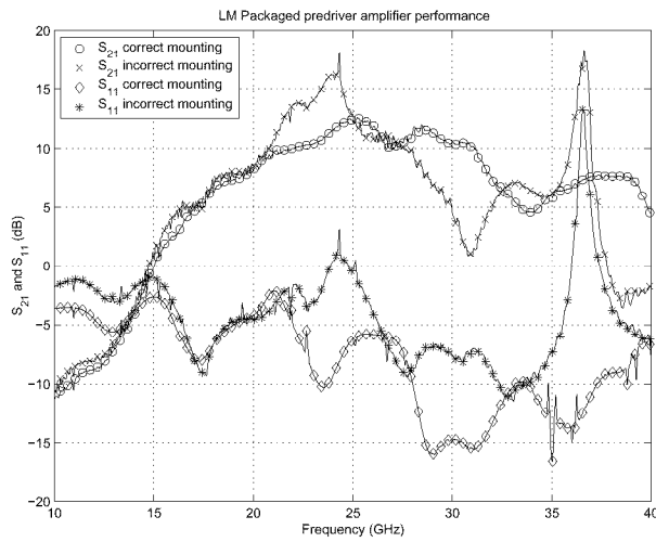
Figure 5: Small signal parameters measurement for correct and incorrect mounting structure.
