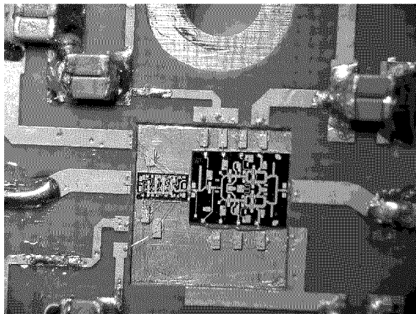
Figure 3: Power stage for the 25.7 GHz transmitter module prototype.
