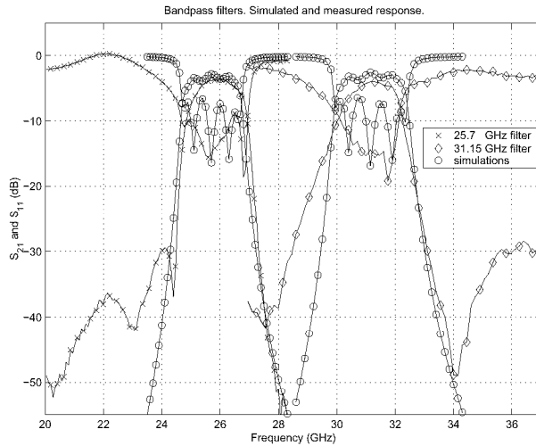
Figure 2: Simulated and measured response of 25.7 GHz and 31.15 GHz filters.
