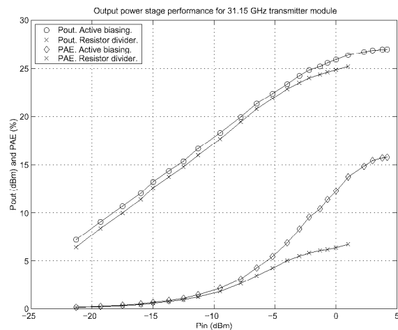
Figure 8: Power stage performance for 31.15 GHz module. Both measurements for the same DC power consumption without RF signal (900 mA @ 3.5 V).
