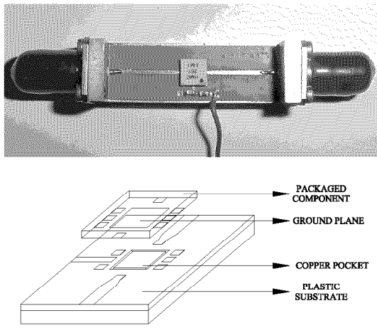
Figure 4: a. Predriver amplifier and measurement fixture. b. Correct ground plane mounting structure.
