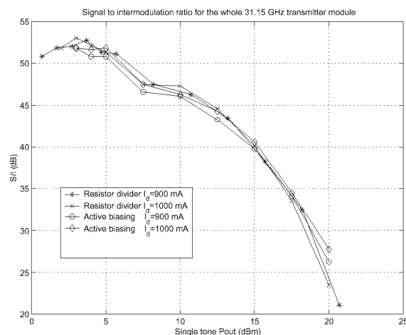
Figure 9: Signal to intermodulation ratio for the whole 31.15 GHz transmitter module.
