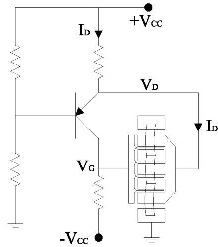
Figure 6: Active biasing network for PAE improvement and avoiding adjustments.
