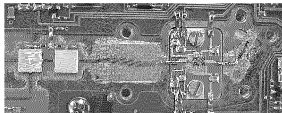
Figure 11: 25.7 GHz transmitter full production module.
